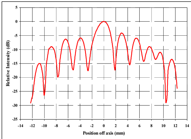
Figure 4. Cross-Axis scan results
