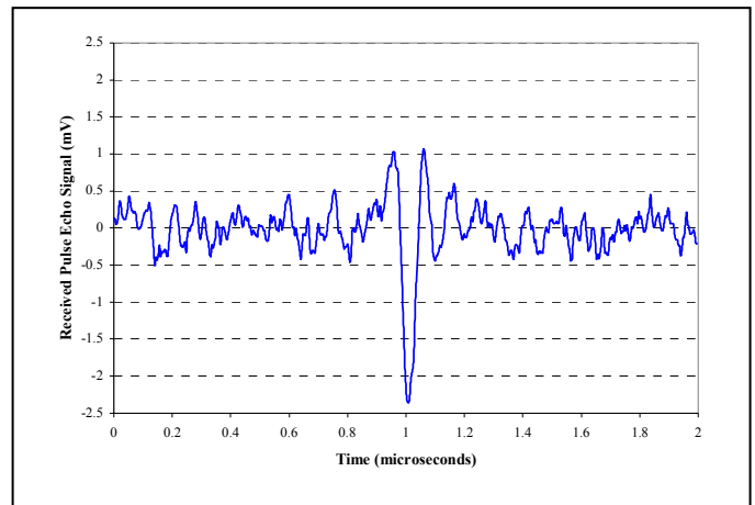
Figure 3. Pulse Echo response to the glass fiber target
