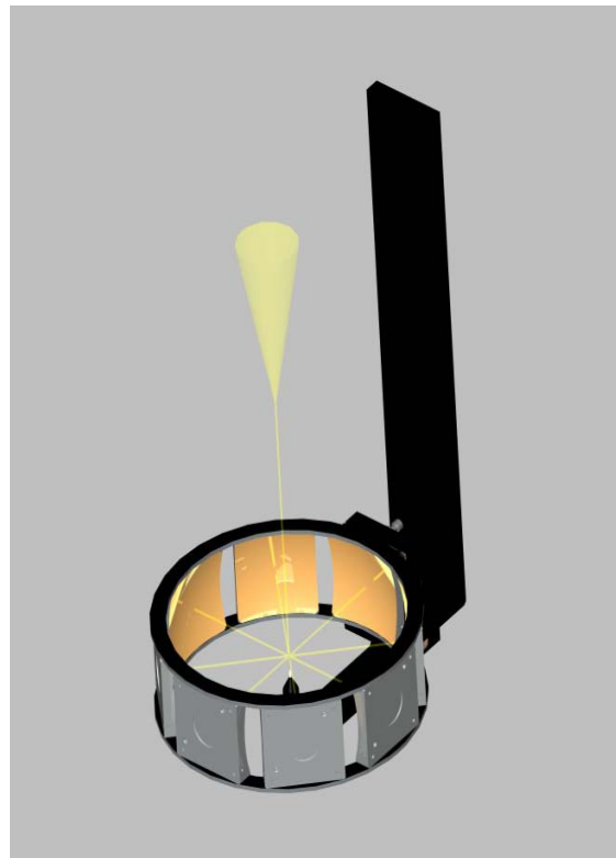
Figure 1. Schematic Diagram of HIFU Hydrophone Concept.
