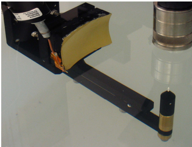
Figure 2. Photograph of the prototype in the water tank. Note the test transducer on the upper right, the PVdF receiver array on the left, and the preamplifier module at the upper left.
